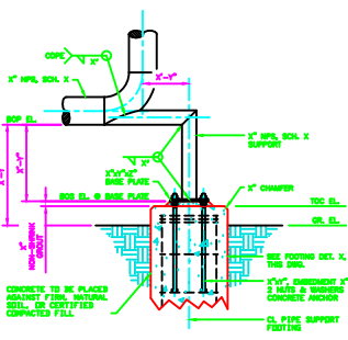
DET. 1 DUMMY SUPPORT WITH BASE PLATE
