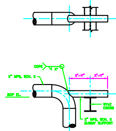
DET. 1 DUMMY PIPE SUPPORT I BEAM SUPPORT
