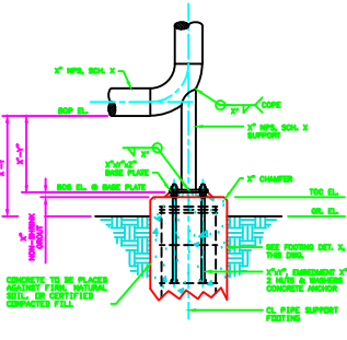
DET. 1 DUMMY SUPPORT WITH BASE PLATE
