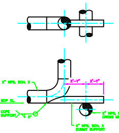
DET. 1 DUMMY PIPE SUPPORT PIPE SUPPORT
