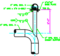
DET. 1 DUMMY SUPPORT WITH U-BOLT
