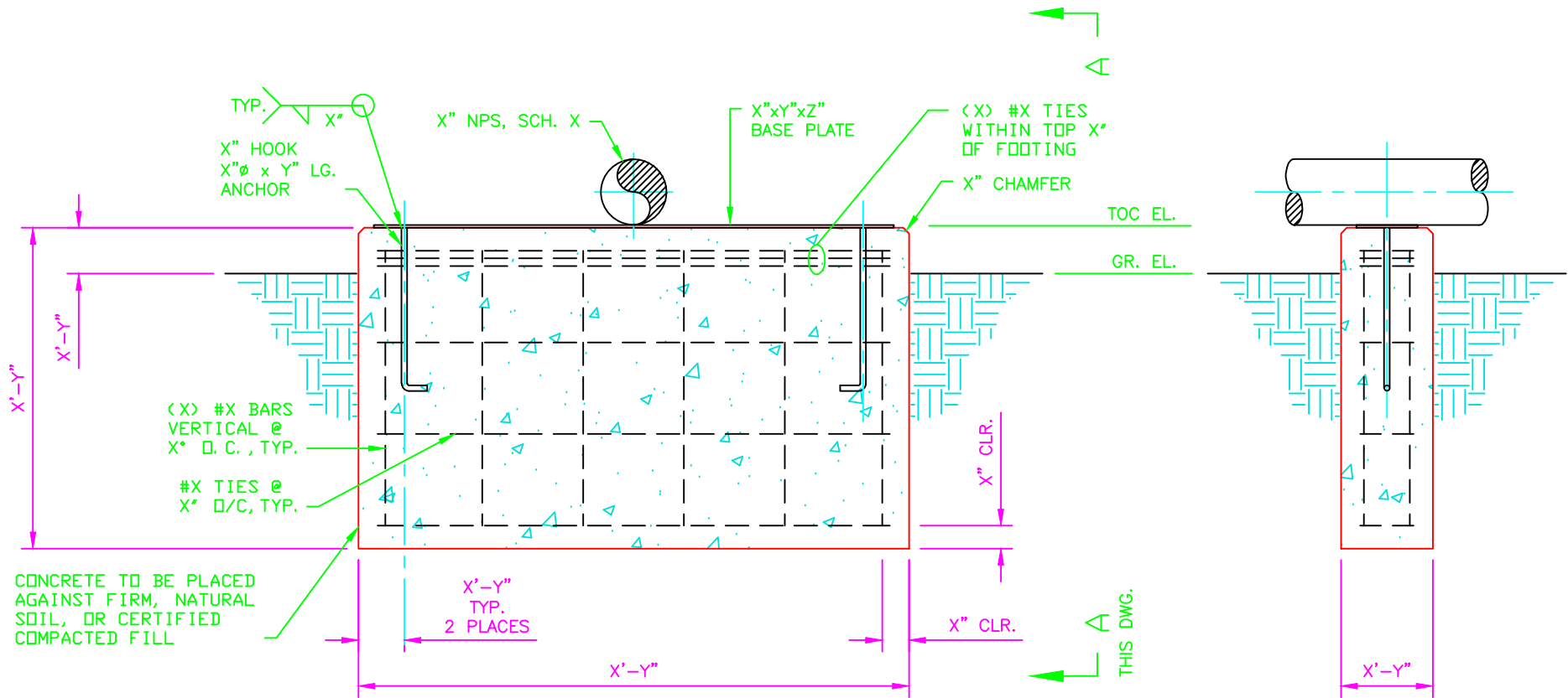
WALL PIPE SUPPORT WITH BASE PLATE
