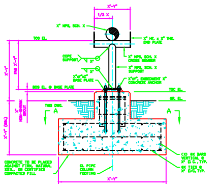
DET. 1 T SPREAD PIPE SUPPORT WITH BASE PLATE
