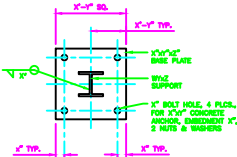
DET. 2 BASE PLATE w/BEAM
