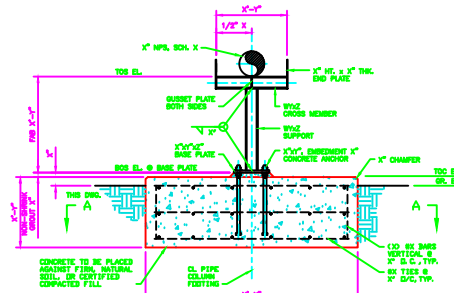
DET. 1 T SPREAD BEAM SUPPORT WITH BASE PLATE
