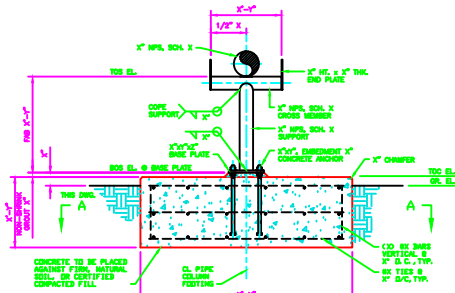
DET. 1 T SPREAD PIPE SUPPORT WITH BASE PLATE
